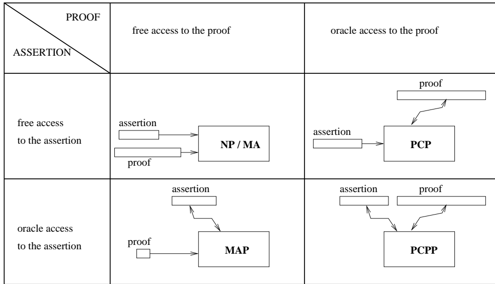
Figure 12.1: A taxonomy of four non-interactive proof systems.
