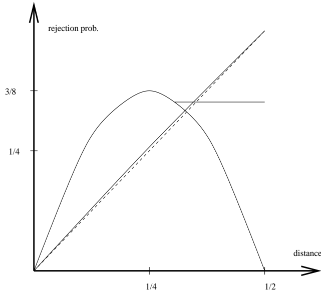
Figure 13.1: The lower bounds that underlie the function \Gamma . The dashed diagonal line represents the bound \varrho(x) \geq x , which is slightly improved by the bound \varrho(x) \geq x + \eta(x) .
