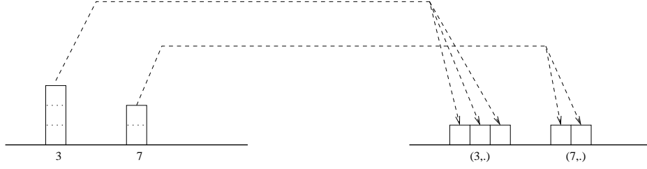
Figure 11.1: The grained-to-uniform filter corresponding to the 5-grained distribution q that satisfies q(3) = 3/5 and q(7) = 2/5 .
