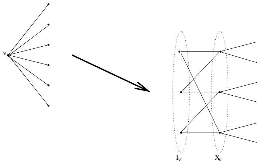
Figure 10.1: The gadget G_v for the case of \bar{d} = 2 and t_v = 3 . The vertex v is replaced by a bipartite graph with sides X_v and I_v , where “X” stands for external and “I” for internal.
