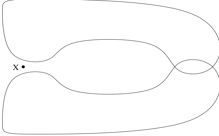
Figure 1.1: Being closed to two sets versus being closed to their intersection
