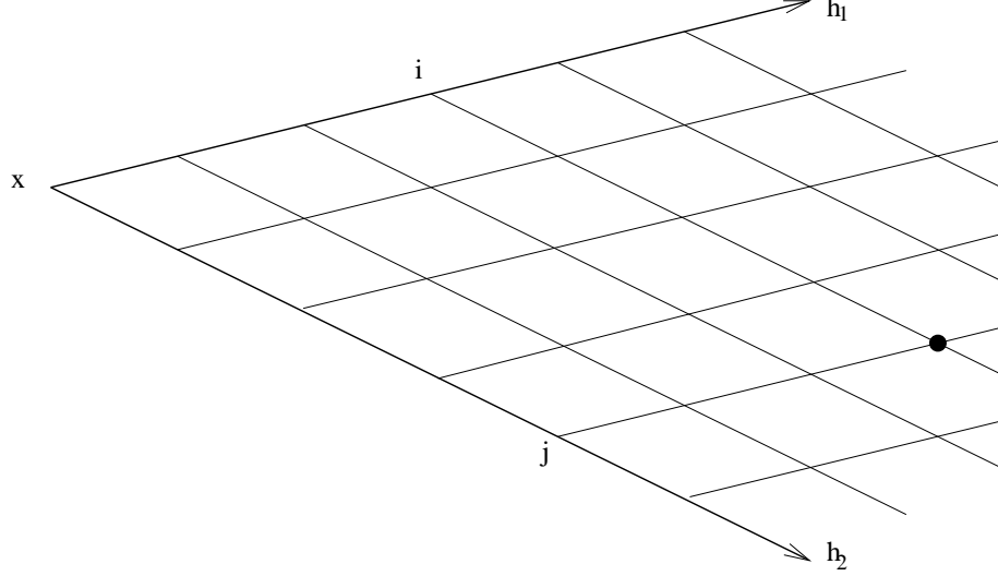
Figure 3.1: The lattice spanned by \bar{h}_1 and \bar{h}_2 , and the point \bar{x} + i\bar{h}_1 + j\bar{h}_2 .
