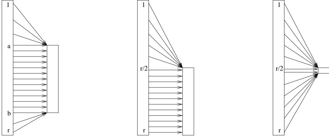
Figure 4.3: The generic filter F_{a,b} (on the left), and the cases of F_{1,0.5r} and F_{0.5r,0.5r+1} .
