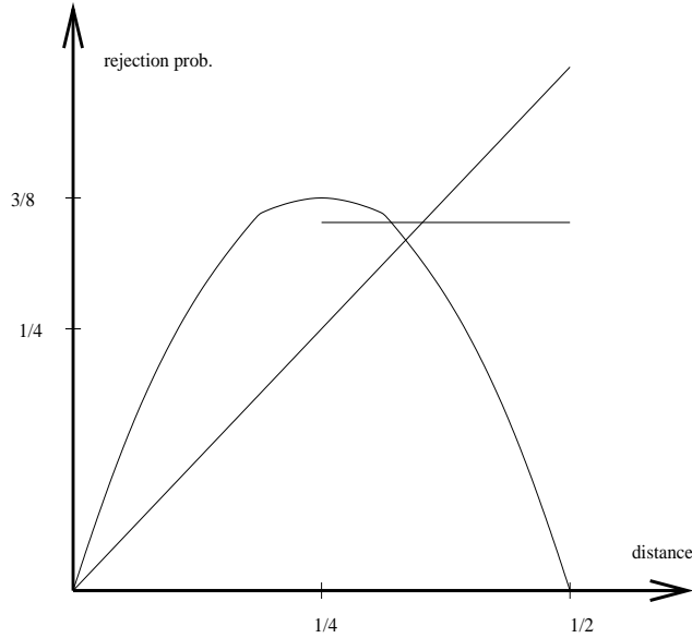
Figure 2.2: The three lower bounds on the rejection probability of f as a function of distance of f from a homomorphism, for H = \text{GF}(2) and G = \text{GF}(2)^m .
