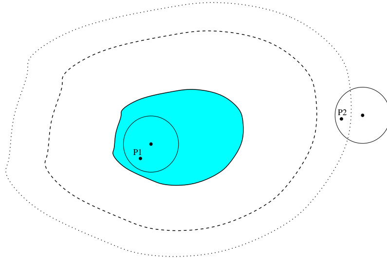
Figure 11.3: The proof of Claim 11.31.1. The shaded region represents \mathcal{D} , and the dashed (resp., dotted) line represents distance \epsilon (resp., \epsilon + \eta ) from \mathcal{D} . The left (resp., right) circle represent the set of distributions that are \eta -close to U_n (resp., to U_{n/2} ), which contains p_1 (resp., p_2 ). In the figure p_2 is depicted as being at distance \delta \in (\epsilon, \epsilon + \eta] from \mathcal{D} , but it may the case that p_2 is (\epsilon + \eta) -far from \mathcal{D} .
