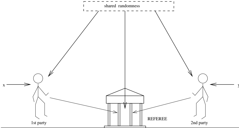
Figure 7.1: The simultaneous communication model.
