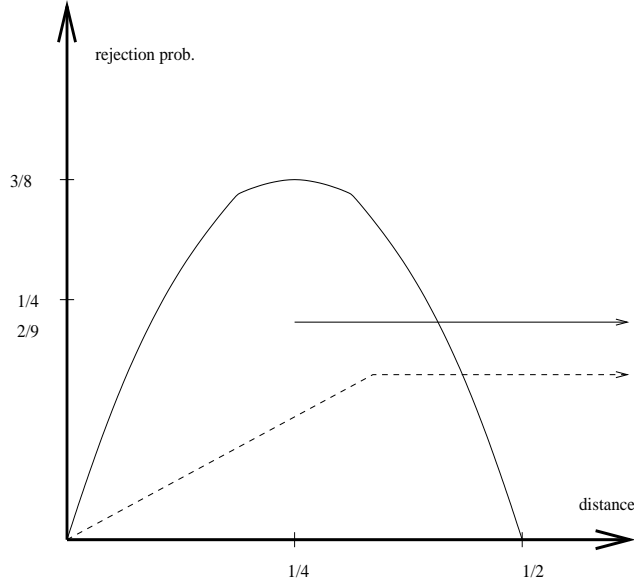
Figure 2.1: The lower bounds on the rejection probability of f as a function of the distance of f from a homomorphism, for general groups. The two solid lines show the bounds underlying \beta(\cdot) , whereas the broken dashed line shows the bound \min(0.5x, 1/6) .
