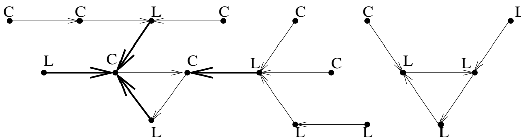
Figure 9.1: A directed graph of heaviest edges and a random choice of values for the vertices. The edges are directed from each vertex to its heaviest neighbor, and the edges that will be contracted are shown by wider arrows.
