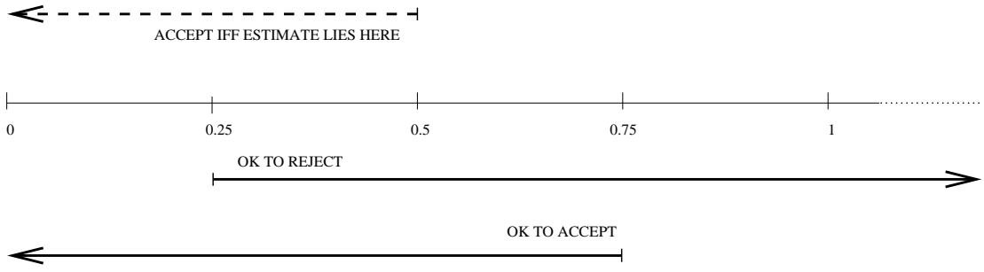
Figure 5.1: Detail for the proof of Theorem 5.7. The algorithmic decision is depicted by a dashed arrow that refers to the estimated value (in multiples of \epsilon 2^\ell ), and the analysis is depicted by solid arrows that refers to the real value of |f^{-1}(1)| .
