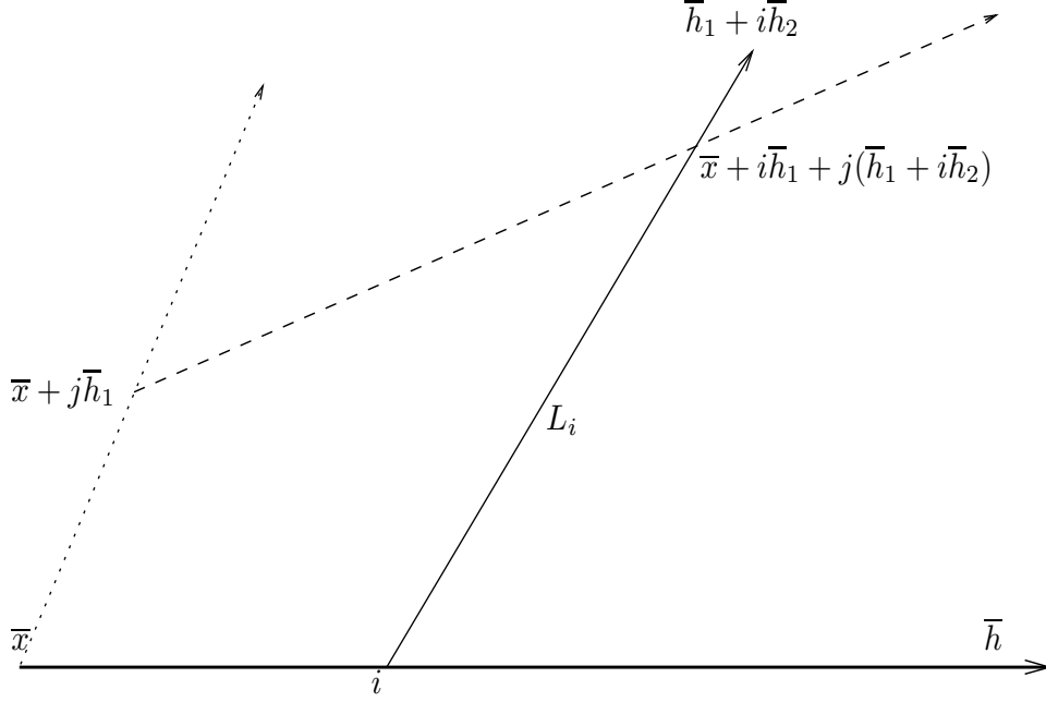
Figure 3.2: The j^{\text{th}} point on the (solid) line L_i = L_{\bar{x} + i\bar{h}, \bar{h}_1 + i\bar{h}_2} is reached as the i^{\text{th}} point on the (dashed) line L_{\bar{x} + j\bar{h}_1, \bar{h} + j\bar{h}_2} , which is totally random. Recall that the line L_{\bar{x}, \bar{h}} is fixed.
