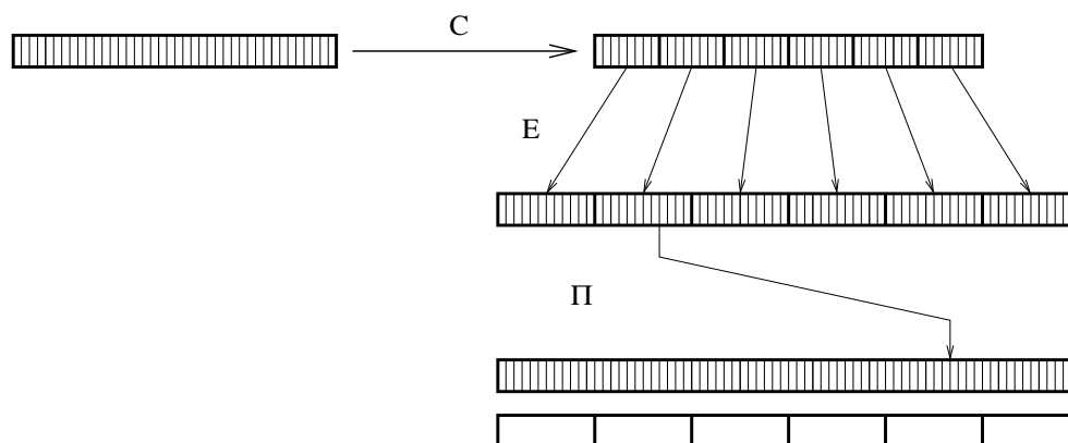
Figure 13.3: Distance amplification for a code C : \Sigma^{40} \rightarrow \Sigma^{48} , when using the encoding E : \Sigma^8 \rightarrow \Sigma^{12} , and a random permutation \pi : [72] \rightarrow [72] , yields a code C' : \Sigma^{40} \rightarrow \Gamma^6 .
