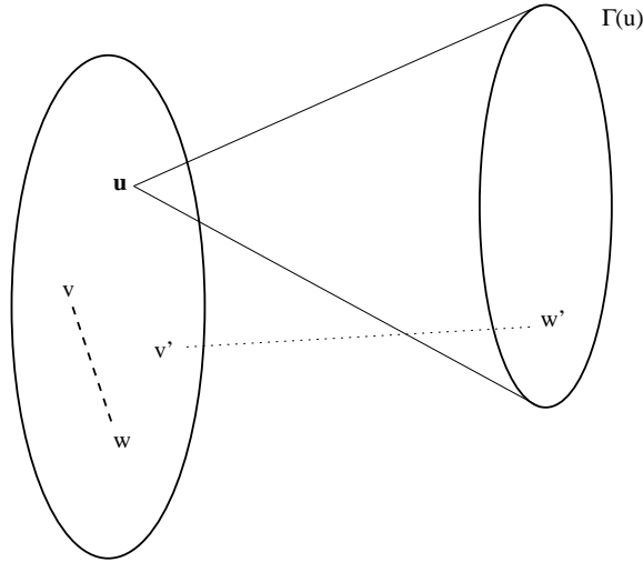
Figure 8.1: The 2-partition imposed by u . The dashed line represents a violating pair connected by an edge, whereas the dotted line represents a violating pair that lacks an edge.
