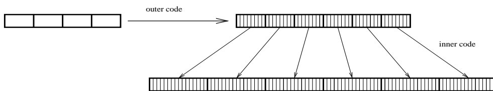
Figure 13.2: Concatenated codes. The outer (resp., inner) encoding is depicted by the horizontal arrow (resp., vertical arrows).
