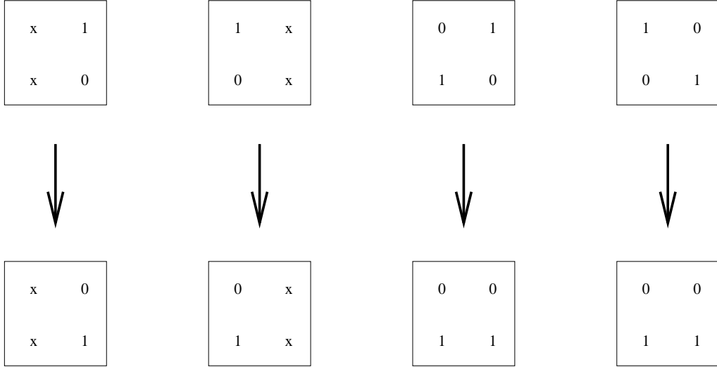
Figure 4.1: The remaining four cases in the proof of Claim 4.2.4. In the first two (leftmost) cases the sorted column equals (xx)^\top , whereas in the other two cases the sorted column is (01)^\top .
