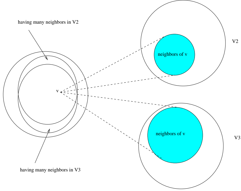
Figure 8.2: The triangles that contain a typical vertex v \in V_1 , which has many neighbors in both V_2 and V_3 . Note that each edge between \Gamma_2(v) and \Gamma_3(v) forms a triangle that contains v .
